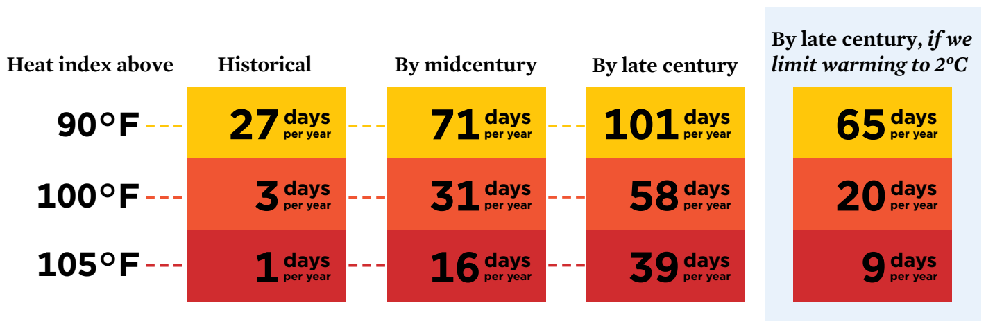
Annual Days of Extreme Heat Per Year in Maryland's 8th District
