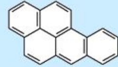
benzo [a] pyrene
