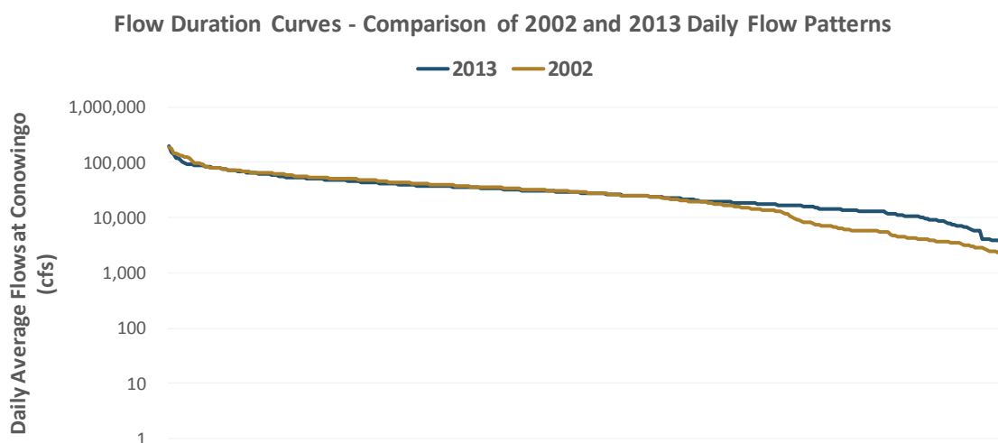
Figure 5: 2002 and 2013 flow duration curves (log scale).
