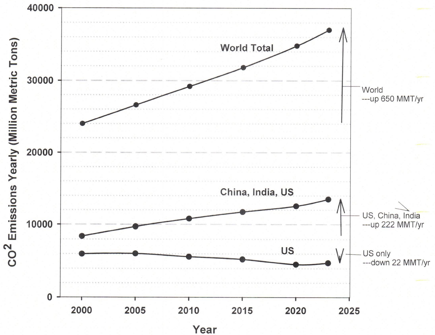
Fig 5 CO 2 Emissions Yearly World Total
